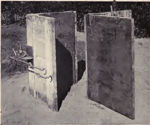
MARK V SHUTTERING.
